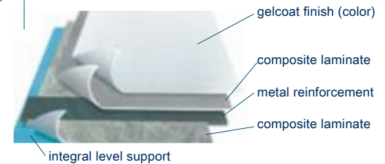
Composite Floor Structure
