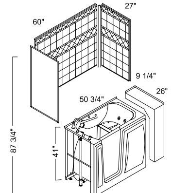
XTW5026 - With three walls and extension
