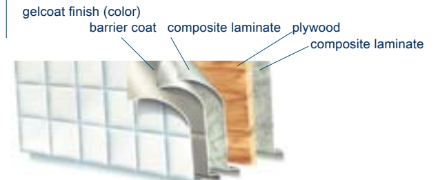
Composite Wall Structure
