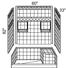
4LDS6032 (also available in 60 x 30)
