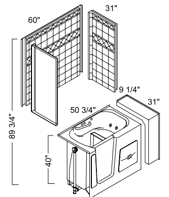
XTOW5030 - With three walls and extension
