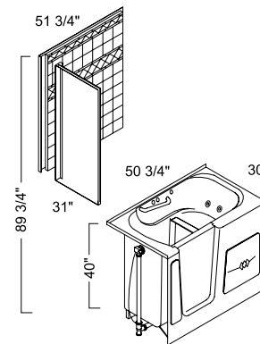
XTOW5030 - With two walls
