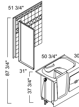
LTOW5030 - With two walls
