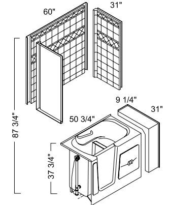
LTOW5030 - With three walls and extension
